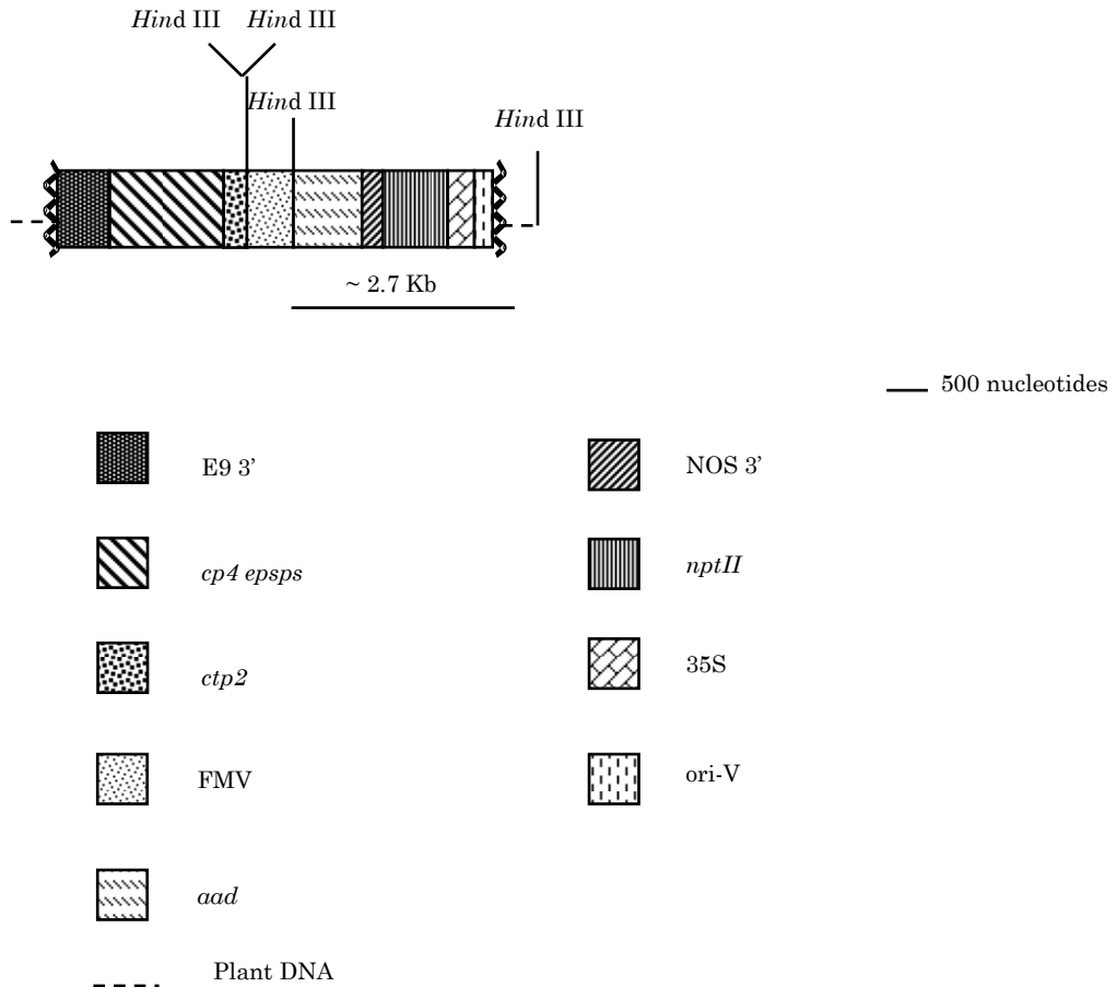
Figure 2 Schematic representation of the insert in MON 1445
